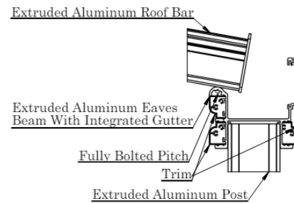
Eaves Beam Roof Bar & Post Section
